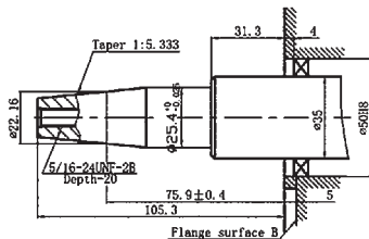
Albero Shaft Mod. G1
